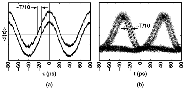
Fig. 5. When the polarization state of the data signal varies, the background nonlinear photocurrent changes, leading to a shift in the timing of the recovered clock. (a) Output of detector versus delay \tau for two extremal cases obtained by adjusting the input polarization state. (b) Superposed eye diagrams for the two extremal cases considered in (a) showing the timing shift due to polarization changes.
