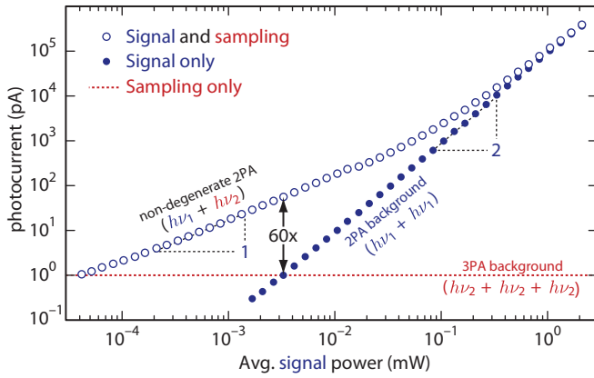
Fig. 2. Measured average photocurrent in GaAs photodiode vs. average signal power, for fixed sampling power of 100 \mu\text{W} .
