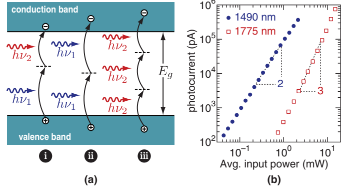
Fig. 1. a) Three dominant nonlinear processes that contribute to photocurrent: (i) nondegenerate 2PA from sampling and signal pulses, (ii) 2PA from signal pulses and (iii) 3PA from sampling pulses. b) The background photocurrent as a function of incident power for \lambda = 1490 and 1775 nm.
