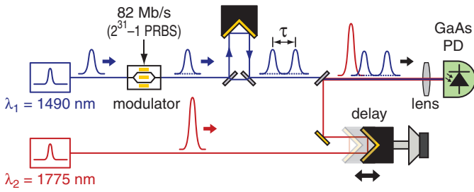
Fig. 4. Experimental setup for optical sampling based on nondegenerate 2PA.
