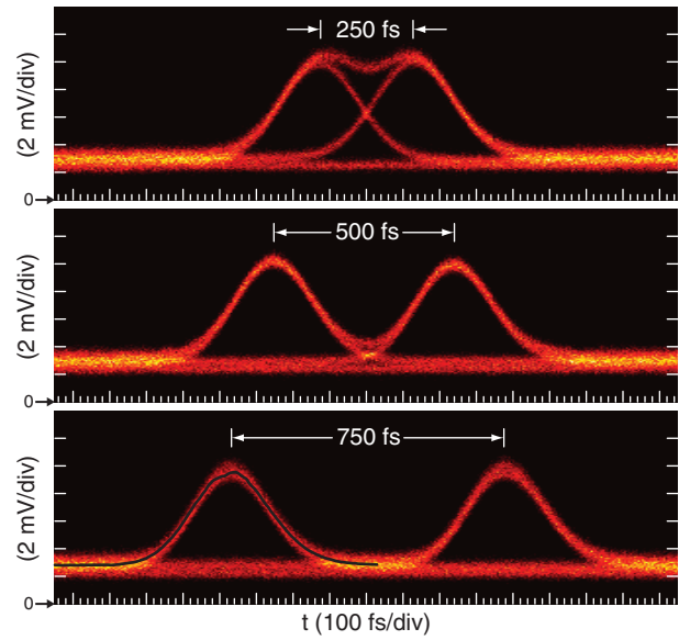
Fig. 5. Measured eye diagram of a on-off keyed signal with inter-symbol spacings of 250, 500, and 750 fs.
