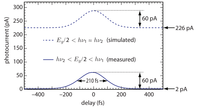
Fig. 3. The cross-correlation between sampling and signal pulses. The solid line represents the measured cross-correlation when h\nu_2 < E_g/2 < h\nu_1 . The dashed line is the simulated cross-correlation that for the case when E_g/2 < h\nu_2 \approx h\nu_1 .
