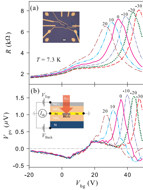
FIG. 1 (color online). Photovoltaic response and resistance of a dual-gated bilayer graphene. (a) Resistance and (b) photovoltaic response as a function of back gate voltage for different top gate voltages at T = 7.3 K and zero bias current. Inset in (a) shows an optical micrograph of the bilayer graphene device. Scale bar, 10 \mu\text{m} . Inset in (b) shows schematic of device geometry and electric-field-effect gating.
