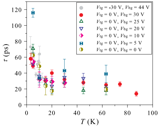
FIG. 4 (color online). Temperature dependence of thermal response time. Thermal time constant \tau of the photovoltaic response vs temperature measured by the pulse coincidence technique for several different dual-gate voltage settings.
