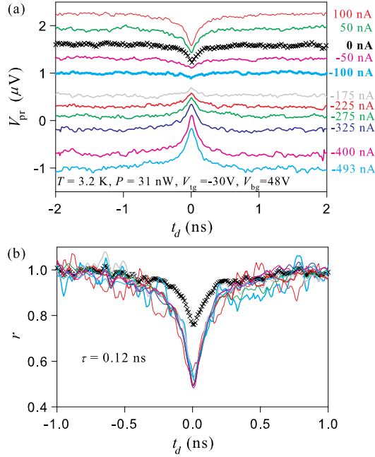
FIG. 2 (color online). Bias current dependence of the pump-probe measurements. Photoresponse from pump-probe laser pulses as a function of time delay t_d at 3.2 K and laser power of 31 nW. The sample is gated to charge neutrality with V_{tg} = -30 V, V_{bg} = 48 V. (a) Bias current I_{dc} dependence of probe-induced photoresponse voltage V_{pr}(t_d) as a function of the probe beam delay time t_d . The I_{dc} = 0 curve is the photovoltaic response. (b) r is the normalized bolometric response \Delta V(I_{dc}) = V(I_{dc}) - V(0) and photovoltaic response V(0) . r = V_{pr}(t_d)/V_{pv}^0 , where V_{pv}^0 = V_{pv}(t_d \gg \tau) . The thermal response time \tau is defined as the half-width at half-maximum of the dip. All dips have a similar time constant \tau = 0.12 \pm 0.01 ns.
