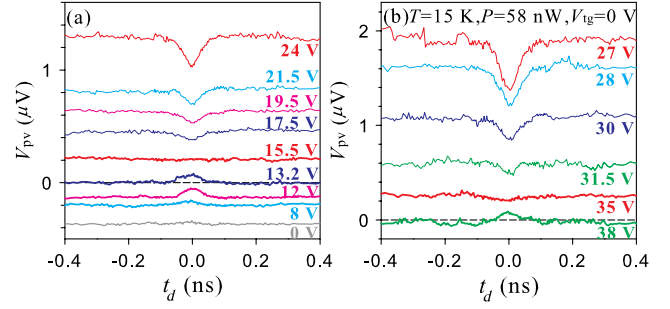
FIG. 3 (color online). Gate voltage dependence of the pump-probe measurements. Pump-probe pulse induced photovoltaic response as a function of time delay at 15 K, laser power of 58 nW, and I_{dc} = 0 . The data were taken at several back gate voltages V_{bg} with zero top gate voltage (a) below and (b) above V_{bg} = 25 V where the maximum photovoltaic response is found. The thin dashed line at V_{bg} = 0 is a guide line. All cusps have the same thermal time constant \tau = 25 \pm 5 ps within error.
