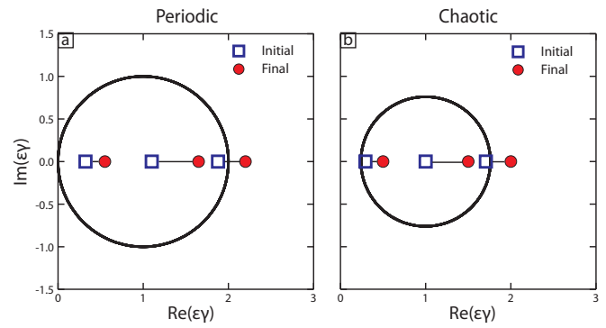
FIG. 8. (Color online) The MSF and Laplacian eigenvalue spectra for the undirected network. (a) Periodic node dynamics ( \beta = 1.35 ). (b) Chaotic node dynamics ( \beta = 3.0 ). The eigenvalues of the original network are represented by \square and those of the network with the link added are represented by \bullet . The black line denotes the zero contour of the MSF: Inside global synchrony is stable; outside it is unstable.
