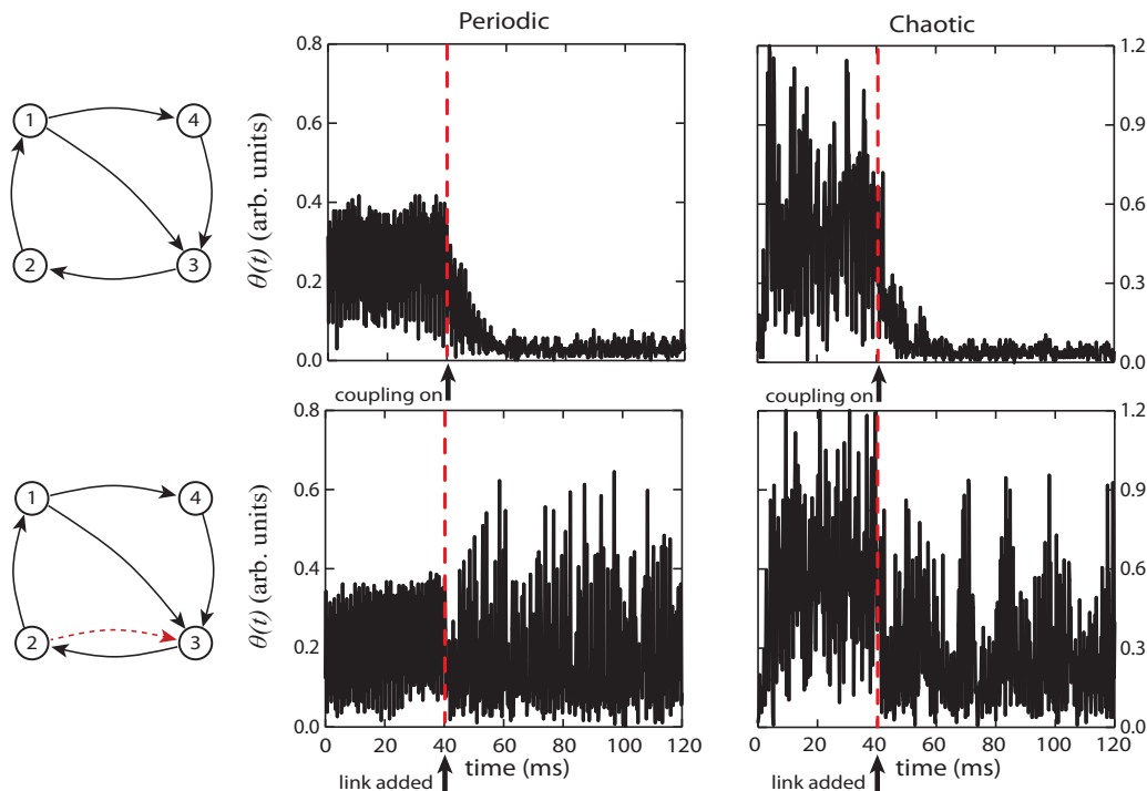
FIG. 3. (Color online) Experimental results for directed network 1. In all cases, the nodes are initially uncoupled. The coupling scheme depicted to the left is implemented at t = 40 ms as indicated by the dashed line. For the periodic case, \epsilon = 0.85 and for the chaotic case \epsilon = 0.49 , which are the same values used in simulation.
